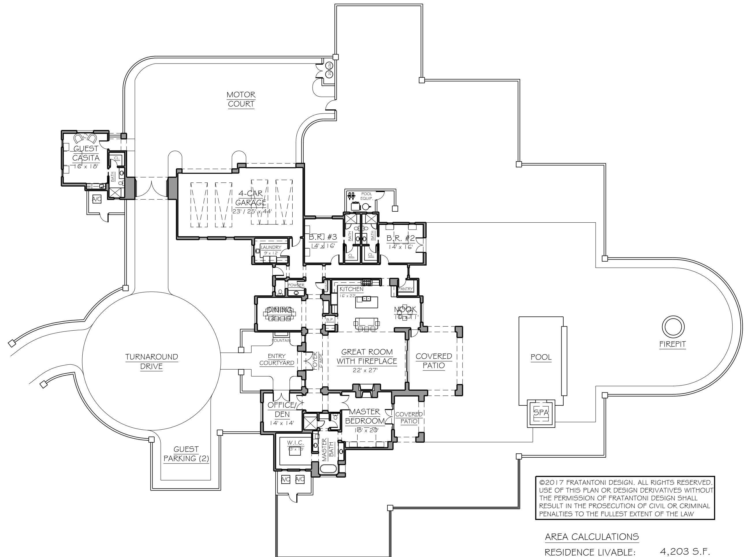
FLOOR PLAN
