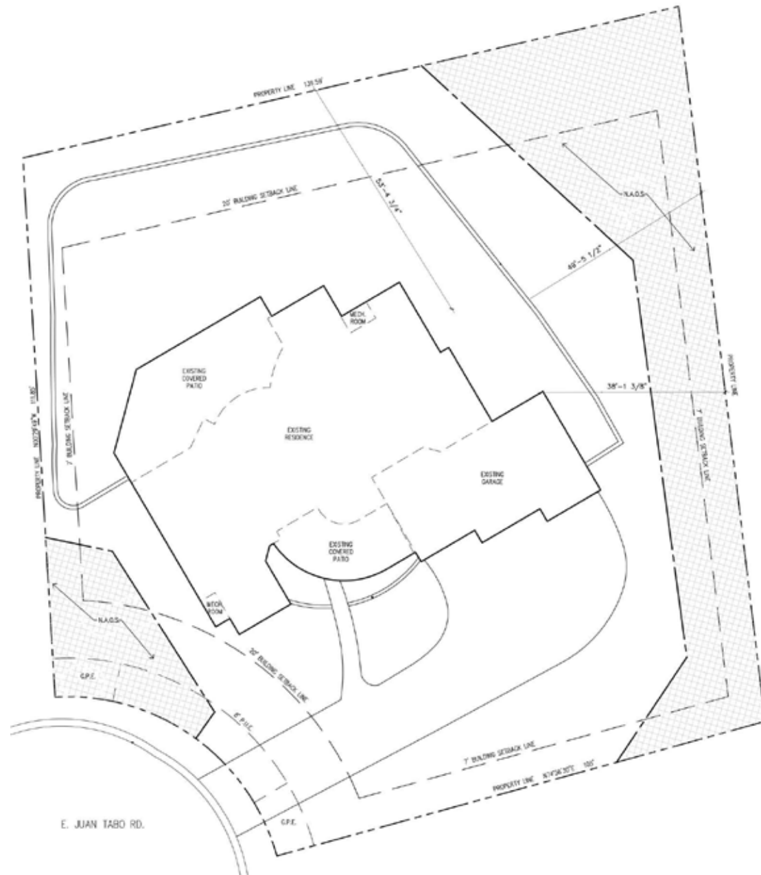
1 ARCHITECTURAL SITE PLAN SCALE: 1" = 10'-0"
